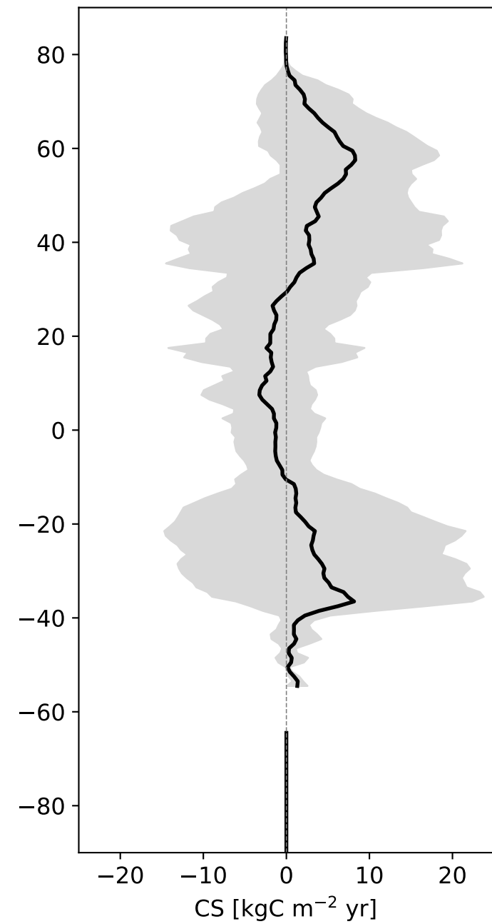
d) CAMS
