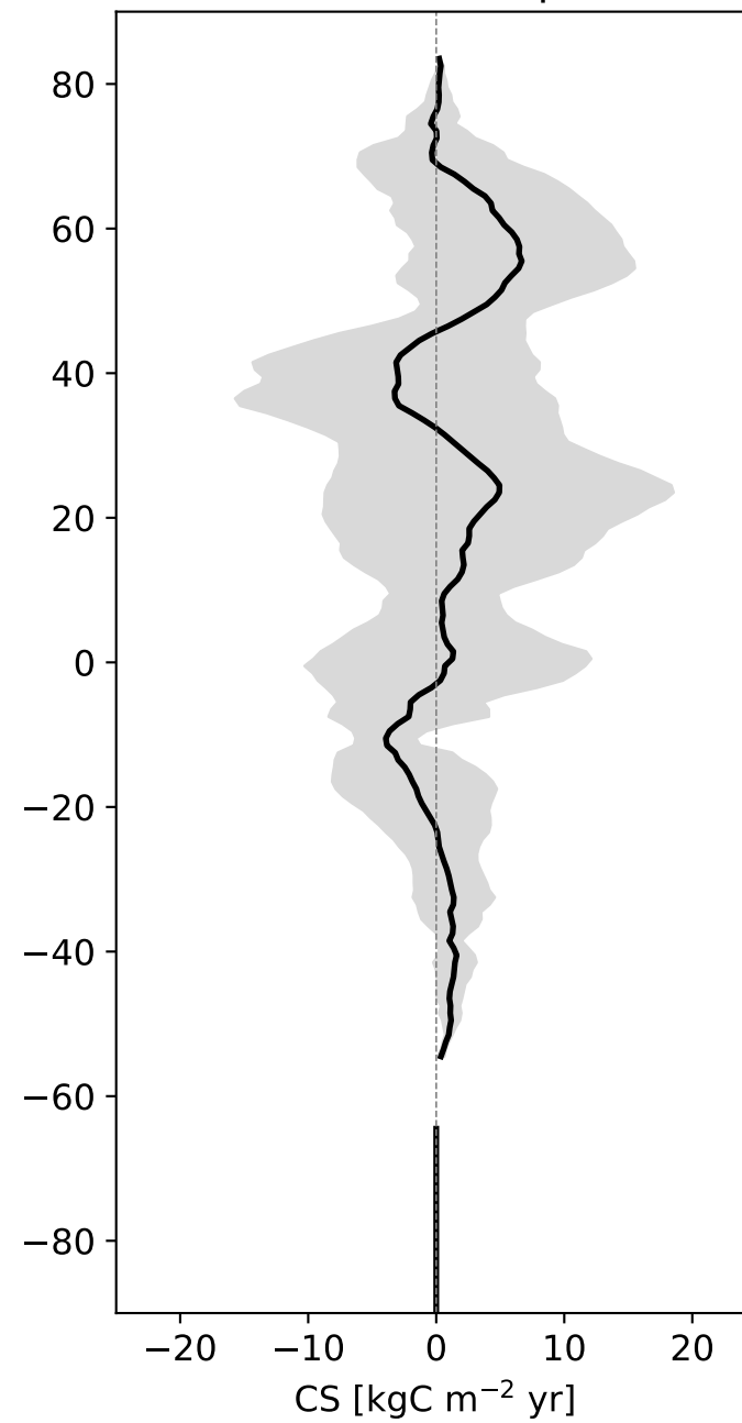
c) CarboScope
